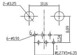
PC BOARD LAYOUT THICKNESS=1.6MM
